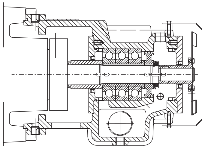
Oil bearing fan cooling
