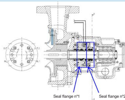
Double seal system as per Plan 55
