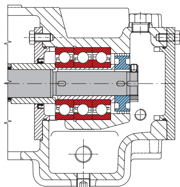
Bearings housing
