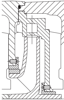
Possible wear rings: single or double on casings, impellers and diffusers
