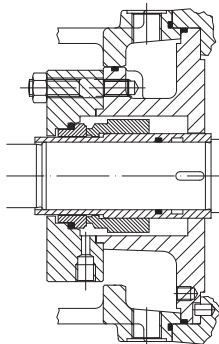
Mechanical seal with coal chamber
