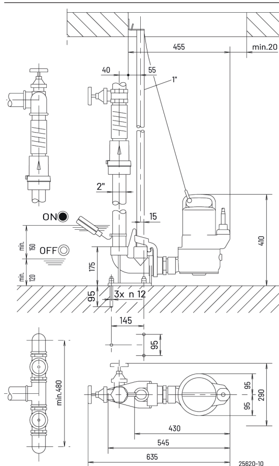
Dimensions GR 50 (mm)
